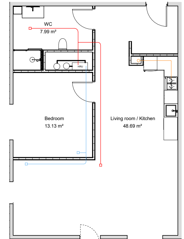
00 All floors Ventilation - Small Apartment 1 : 100
