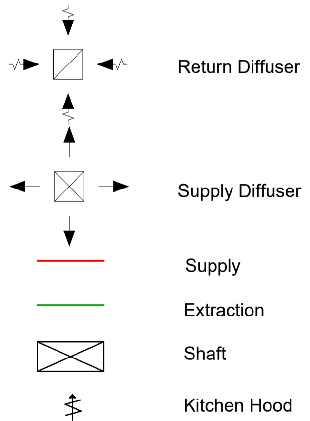
Legend Ventilation Plan Basement
